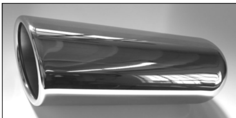
4" & 5" ROLLED ANGLES POLISHED STAINLESS Stock No. Size-Length Slip Over SRA412 4" x 12" 2 1/2" SRA418 4" x 18" 2 1/2" SRA518 5" x 18" 4"
