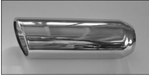
3" ROLLED ANGLES POLISHED STAINLESS Stock No. Size-Length Slip Over SRA309 3" x 9" 2" SRA318 3" x 18" 2 1/4"
