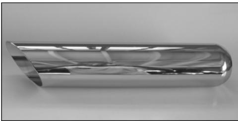
3" & 3 1/2" ANGLE CUTS BLACK STAINLESS Stock No. Size-Length Slip Over BA3018 3" x 18" 2 1/4" BA3518 3 1/2" x 18" 2 1/2" BA3524 3 1/2" x 24" 2 1/2"
