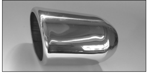
ROLLED OVAL ANGLE POLISHED STAINLESS Stock No. Width-Height-Length Slip Over SRO350 3 3/4" x 3 1/4" x 6" 2 1/4"
